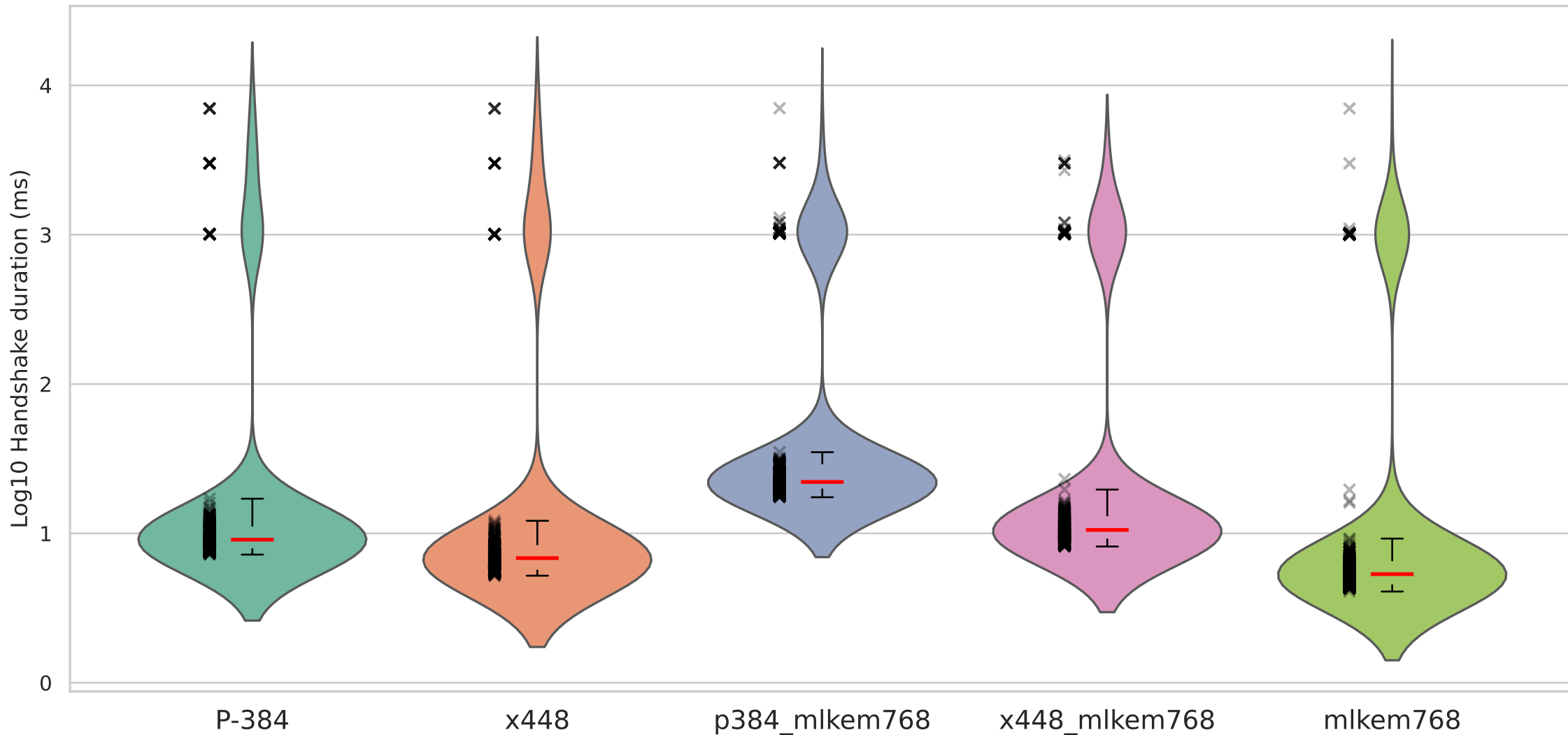
Handshake duration on QUIC with secp384r1 signature algorithm
